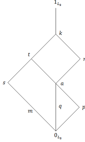
Figure 3: The lattice L_3
