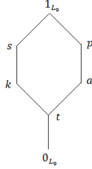
Figure 9: The lattice L_9
