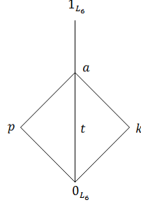
Figure 6: The lattice L_6
