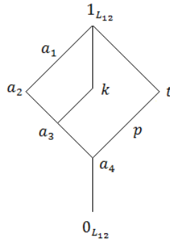
Figure 12: The lattice L_{12}
