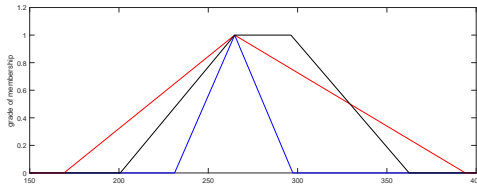
Figure 9: Optimum value for k = 2 as a HFN in Example 5.1 by using the new arithmetic operations.
