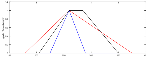
Figure 10: Optimum value for k = 3 as a HFN in Example 5.1 by using the new arithmetic operations.
