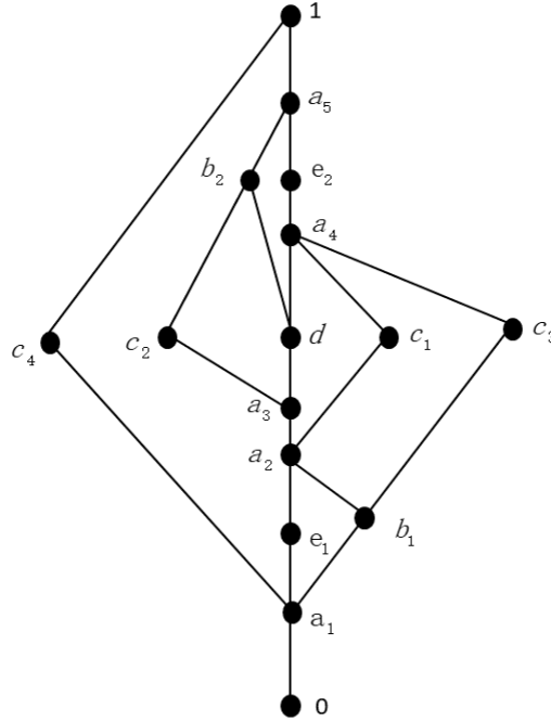
Figure 2: The bounded lattice L_1
